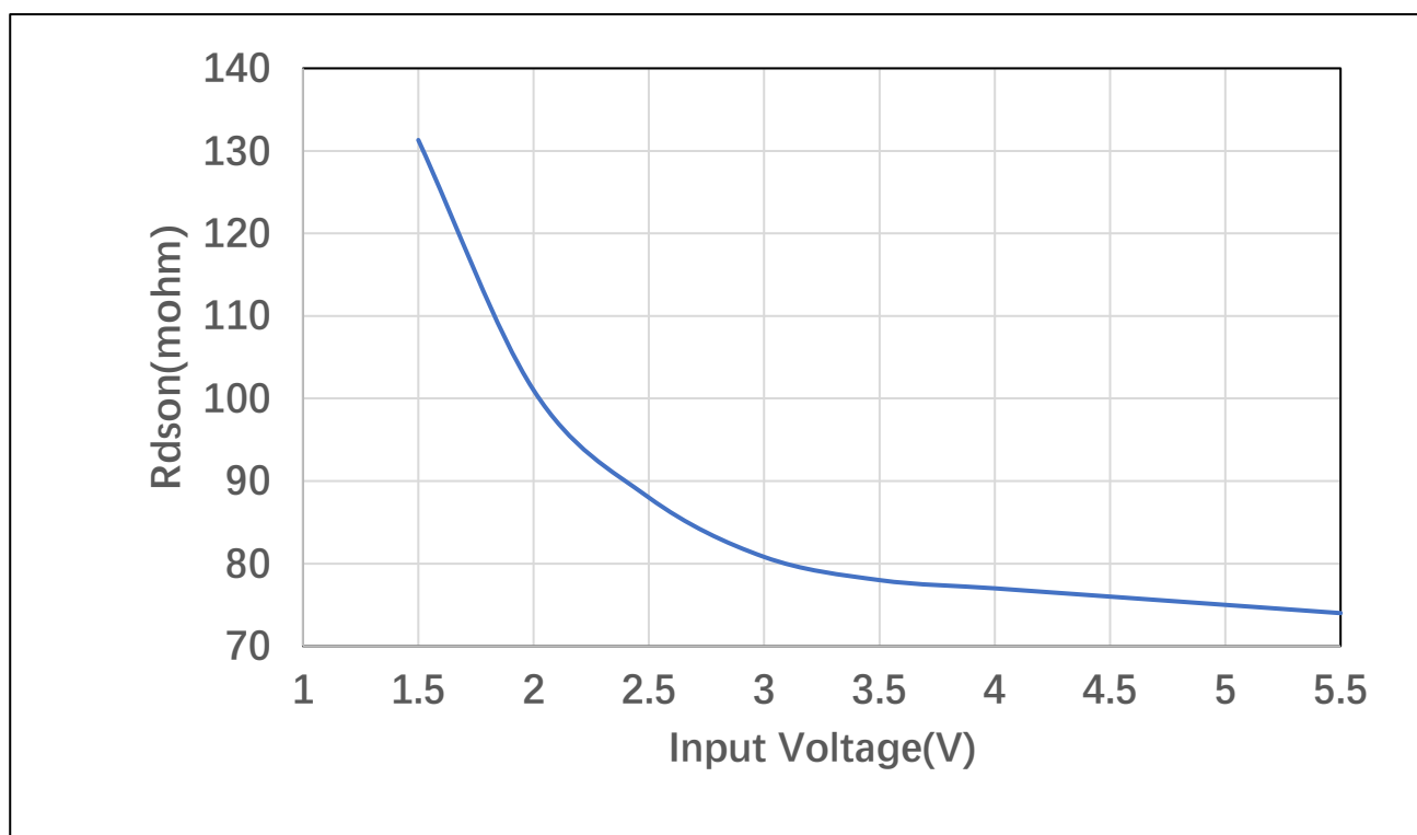
R_{ON} vs. V_{IN} ( V_{EN}=V_{IN}, I_{LOAD}=200mA )
