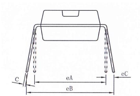
SIDE VIEW 侧视图
