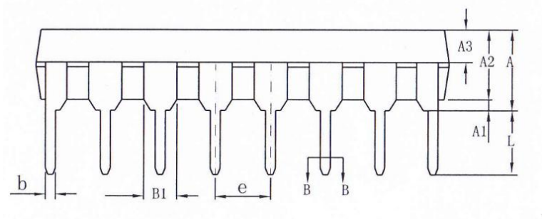
SIDE VIEW 侧视图
