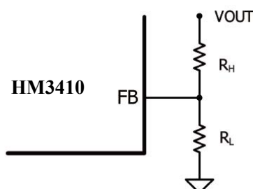
Figure 1 Feedback Network
