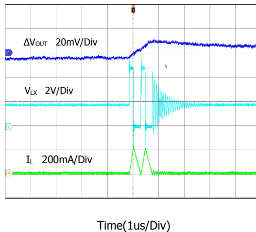
Output Ripple
