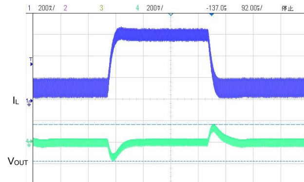
(16) Load Transient(VIN=50.0V,VOUT=12V,IOUT=0.1→0.6A)
